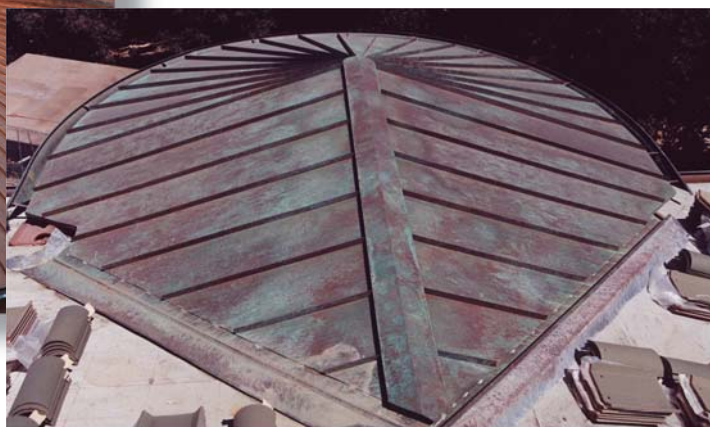
20 oz copper roof over radius copper gutter
