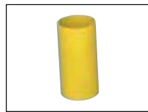
METAL SLEEVE Measures 4" high x 2" O.D. For flush concrete mount Model BVDKR-P107
