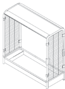
32" (81 cm) X-CART On-rail only Cart features lateral casters 79" H (201 cm) 32" W (81 cm) 78" L (198 cm) 250 lbs (114 kg)
