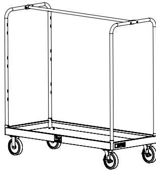
ONBOARD CARGO CART 72.5" (184 cm) L x 31.5" (80 cm) W x 70.5" (179 cm) H Available with hard or pneumatic casters
