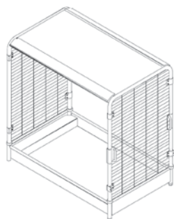
48" (122 cm) X-CART On-rail only Cart features lateral casters 79" H (201 cm) 48" W (122 cm) 78" L (198 cm) 334.88 lbs (152 kg)
