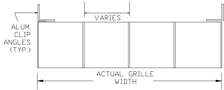
HORIZONTAL SECTION
