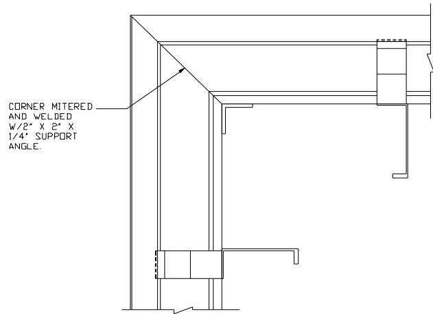
TYPICAL MITERED CORNER SECTION
