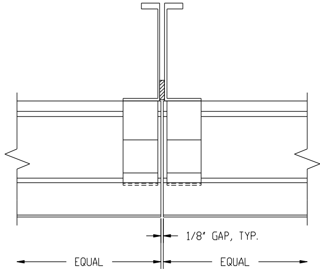
INVISIBLE MULLION DETAIL
