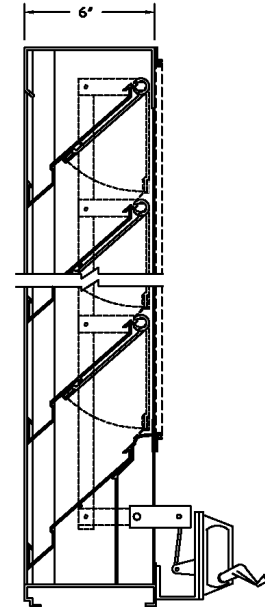
Vertical Section
