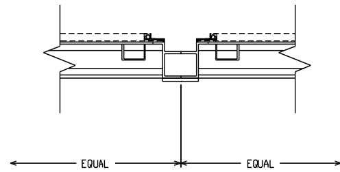
VISIBLE MULLION DETAIL
