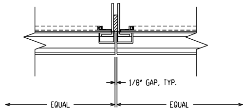
INVISIBLE MULLION DETAIL
