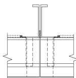
Invisible Vertical Mullion
