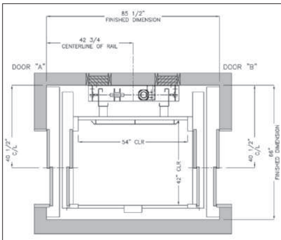
Opposite Opening
