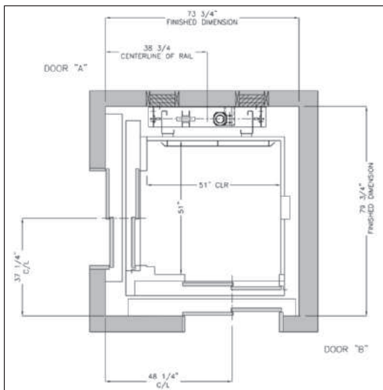
90 Degree Opening
