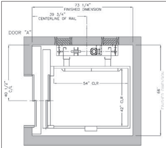
Single Opening
