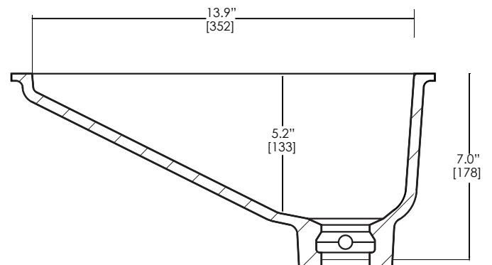
SIDE CROSS-SECTION
