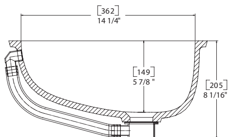
SIDE CROSS-SECTION
